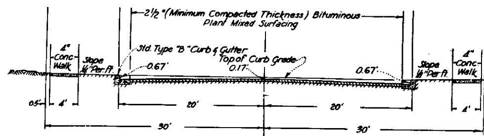
TYPICAL X-SECTION RALSTON AVE. SCALE: 1" = 6'
